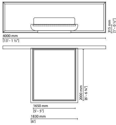
027 413 — Bed 4000x1200 mm (mattress 1650x2000 mm)
