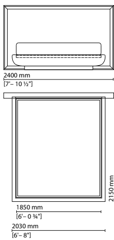
027 412 — Bed 2400×1400 mm (mattress 1850×2150 mm)
