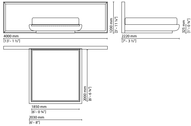
027 414 — Bed 4000x1200 mm (mattress 1850x2000 mm)
