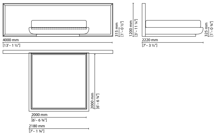
027 415 — Bed 4000x1200 mm (mattress 2000x2000 mm)
