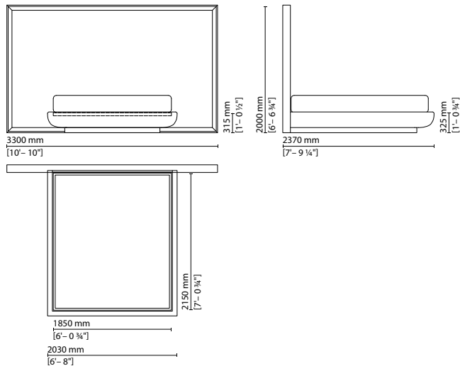
027 406 — Bed 3300×2000 mm (mattress 1850×2150 mm)
