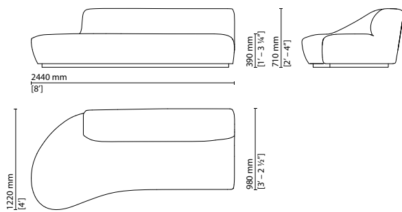
012 015 — Long left end element without armrest
