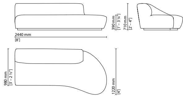
012 016 — Long right end element without armrest
