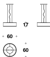
LLL (55) SOSPENSIONE / SUSPENSION Ø 60x17H.cm Ø 23 2/3x6 3/4H."
