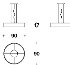
LLL (56) SOSPENSIONE / SUSPENSION Ø 90x17H.cm Ø 35 1/3x6 3/4H."
