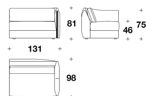
DLS (EGD) - DLS (EGS) BIG : ELEMENTO 1 POSTO CON BRACCIOLO DX O SX / 1 SEATER ELEMENT WITH RIGHT OR LEFT ARMREST 131x98x81H. - H.S.46cm 51 2/3x38 2/3x32H. - H.S.18"
