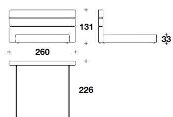
NBR (BLE7) LETTO PER MATERASSO / BED FOR MATRASS 200x200 - 260x226x131H. - H.B.33 cm 78 2/3x78 2/3 - 102 1/3x89x51 2/3H. - H.B.13 "
