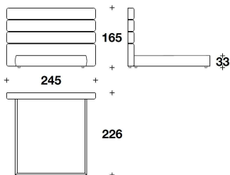
NBR (LE2) HIGH : LETTO PER MATERASSO / BED FOR MATRASS 185x200 - 245x226x165H. - H.B.33 cm 73x78 2/3 - 96 1/3x89x65H. - H.B.13 "
