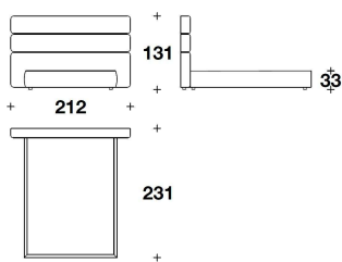
NBR (BQUSA) QUEEN USA : LETTO PER MATERASSO / BED FOR MATRASS 152x205 - 212x231x131H. - H.B.33 cm 60x80 2/3 - 83 1/3x91x51 2/3H. - H.B.13 "
