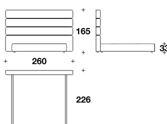
NBR (LE7) HIGH : LETTO PER MATERASSO / BED FOR MATRASS 200x200 - 260x226x165H. - H.B.33 cm 78 2/3x78 2/3 - 102 1/3x89x65H. - H.B.13 "
