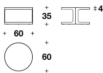
TCV (04) COFFEE TABLE Ø 60x35H.cm Ø 23 2/3x13 3/4H."
