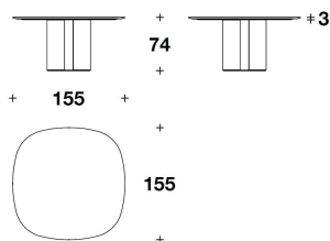
TTV (30M) TAVOLO QUADRATO / SQUARE TABLE 155x155x74H. - THK.3cm 61x61x29H. - THK.1 3/16"
