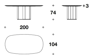
TTV (31M) TAVOLO RETTANGOLARE / RECTANGULAR TABLE 200x104x74H. - THK.3cm 78 2/3x41x29H. - THK.1 3/16"
