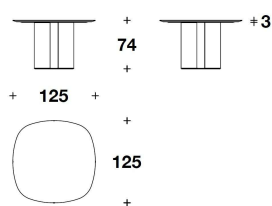
TTV (29M) TAVOLO QUADRATO / SQUARE TABLE 125x125x74H. - THK.3cm 49 1/3x49 1/3x29H. - THK.1 3/16"
