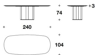
TTV (32M) TAVOLO RETTANGOLARE / RECTANGULAR TABLE 240x104x74H. - THK.3cm 94 1/3x41x29H. - THK.1 3/16"
