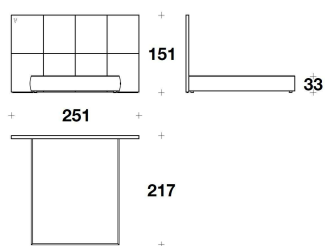
SLE (LE1) LETTO PER MATERASSO / BED FOR MATTRESS 165x200 - 251x217x151H. - H.B.33 cm 65x78 2/3 - 98 2/3x85 1/3x59 1/3H. - H.B.13 "
