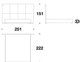
SLE (KUSA) KING USA : LETTO PER MATERASSO / BED FOR MATTRESS 195x205 - 251x222x151H. - H.B.33 cm 76 2/3x80 2/3 - 98 2/3x87 1/3x59 1/3H. - H.B.13 "
