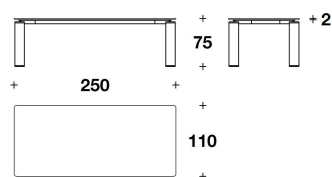
VTB (03) TAVOLO RETTANGOLARE / RECTANGULAR TABLE 250x110x75H. - THK.2 cm 98 1/3x43 1/3x29 2/3H. - THK.13/16 "
