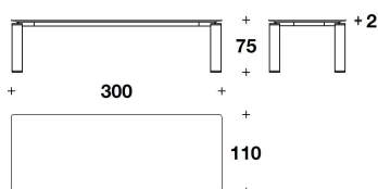
VTB (04) BIG : TAVOLO RETTANGOLARE / RECTAGULAR TABLE 300x110x75H. - THK.2 cm 118x43 1/3x29 2/3H. - THK.13/16 "
