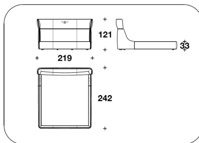
LB1 (LE2) LETTO PER MATERASSO / BED FOR MATTRESS 185x200 - 219x242x121H. - H.B.33cm 73x78 2/3 - 86 1/3x95 1/3x47 2/3H. - H.B.13"
