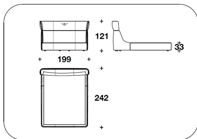
LB1 (LE1) LETTO PER MATERASSO / BED FOR MATTRESS 165x200 - 199x242x121H. - H.B.33cm 65x78 2/3 - 78 1/3x95 1/3x47 2/3H. - H.B.13"
