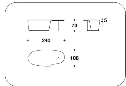
BTV (19PE) TOP SYCAMORE - BURR WALNUT : SCRIVANIA DX O SX / RIGHT OR LEFT WRITING-DESK L.240x108x73H. - 247x246x73H.cm L.94 1/3x42 2/3x28 2/3H. - 97 1/3x97x28 2/3H."
