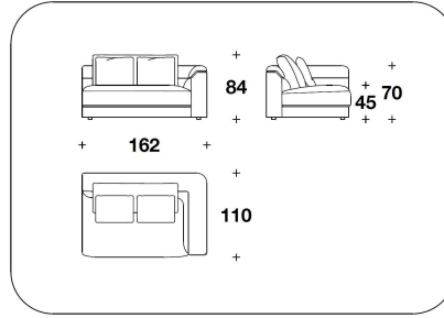
TTN (EDX) - TTN (ESX) MAXI : ELEMENTO 1 POSTO CON BRACCIOLO DX O SX / 1 SEATER ELEMENT WITH RIGHT OR LEFT ARMREST 162x110x84H. - H.S.45 cm 63 2/3x43 1/3x33H. - H.S.17 3/4 "
