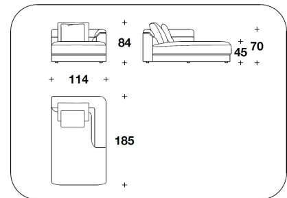
TTN (CLD) - TTN (CLS) CHAISE LONGUE DX O SX / RIGHT OR LEFT CHAISE LONGUE 114x185x84H. - H.S.45 cm 45x73x33H. - H.S.17 3/4 "
