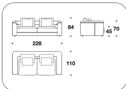
TTN (D3) DIVANO 3 POSTI / 3 SEATER SOFA 228x110x84H. - H.S.45 cm 89 2/3x43 1/3x33H. - H.S.17 3/4 "
