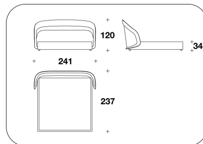
RMG (LE7) LETTO PER MATERASSO / BED FOR MATTRESS 200x200 - 241x237x120H. - H.B.34 cm 78 2/3x78 2/3 - 95x93 1/3x47 1/3H. - H.B.13 2/4 "
