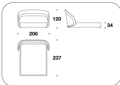
RMG (LE1) LETTO PER MATERASSO / BED FOR MATTRESS 165x200 - 206x237x120H. - H.B.34 cm 65x78 2/3 - 81x93 1/3x47 1/3H. - H.B.13 2/4 "
